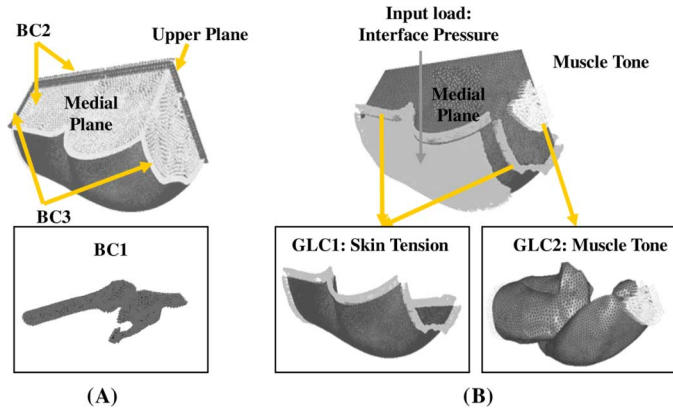
Fig. 3. Boundary and loading conditions used in the FE model. (A) Boundary conditions (BC). BC1: The femur and the pelvis were assumed as rigid bodies and constrained to obviate rigid body motion; BC2: The upper plane and the medial plane were constrained against the anterior–posterior and medial–lateral motions; BC3: Ends of tissues that connect to the rest of the body (distal end to thighs, proximal end to lumbar region) were constrained against longitudinal motions. (B) General loading conditions (GLC) and the input load (Specific loading condition) for the model. GLC1: A “skin initial strain” was applied into the skin layer of the FE model; GLC2: A “muscle tone,” which was 1% of maximal muscle force estimated from F_{\max} = \sigma_{\max} \times \text{PCSA} , was applied along the line of action of each muscle. In the above equation, \sigma_{\max} is the maximal muscle tension [22]; Input load (specific loading condition): an interface pressure of 20.34 kPa was applied to the buttock sitting surface of the model. (a) Boundary conditions (b) Loading conditions.
